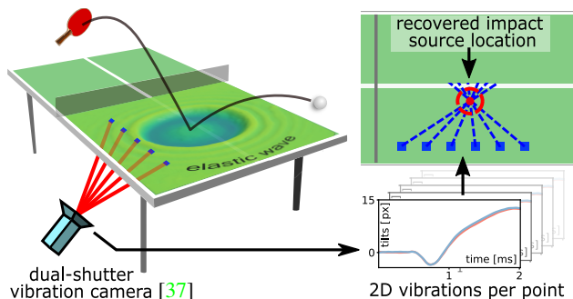
Figure 1. When physical objects interact, like a ping pong ball bouncing off the table, they create minute vibrations that propagate through the objects’ surfaces and interiors. The transient vibrations that occur immediately on impact, exaggerated here for visualization, carry information about the impact source location. We image the surface vibrations at a sparse set of locations using the imaging system of Sheinin et al. [37]. We model the elastic wave propagation and recover the impact source locations without a direct line-of-sight on the impacted surface. Visit the project page for videos of results [1].
